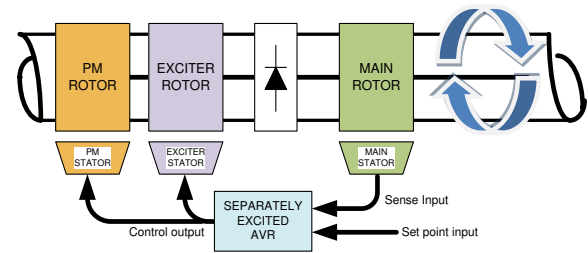
Gambar 7 Separate excitation
