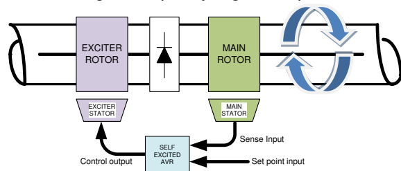
Gambar 6 Self exciter
