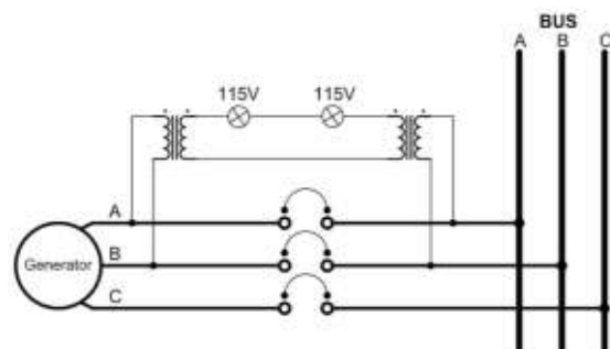
Gambar 3 Indikator lampu sama fasa
