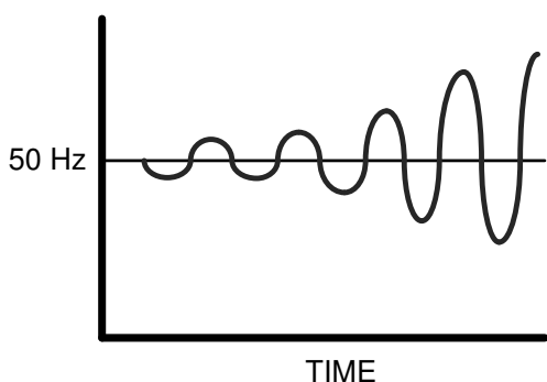
Gambar 8 Curva respon governor tanpa droop
