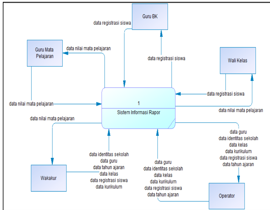
Gambar 3. DFD Level 0
