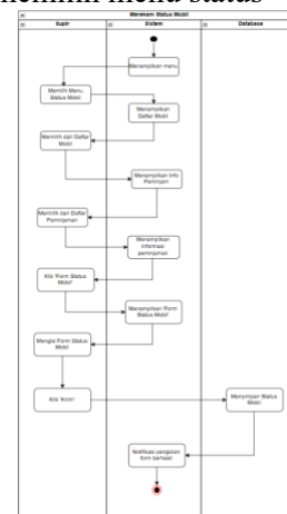
Gambar 5. Activity Diagram Merekam Status Mobil
