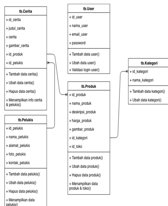
Gambar 4. Class Diagram
