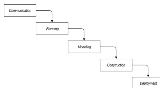
Gambar 1. Metode Waterfall
